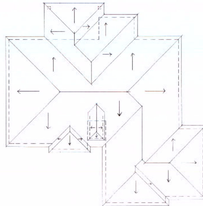
ROOF PLAN \frac{1}{8} " = 1'-0" SLOPES 10/12
